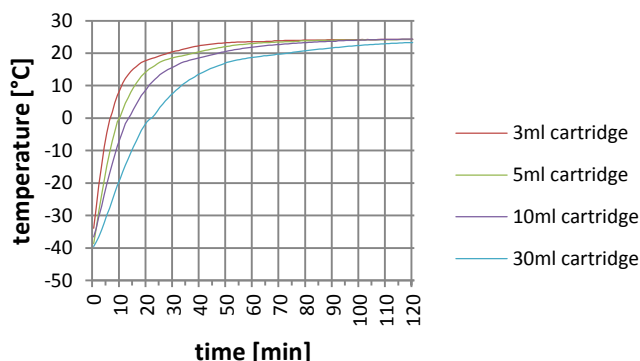
Thawing curve -40°C
